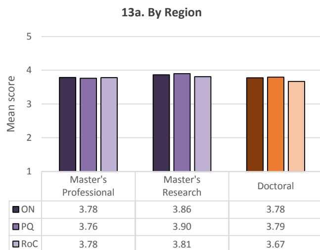
Figure 13: Teaching Benchmark
